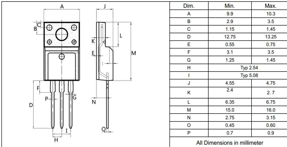
TO-220F
