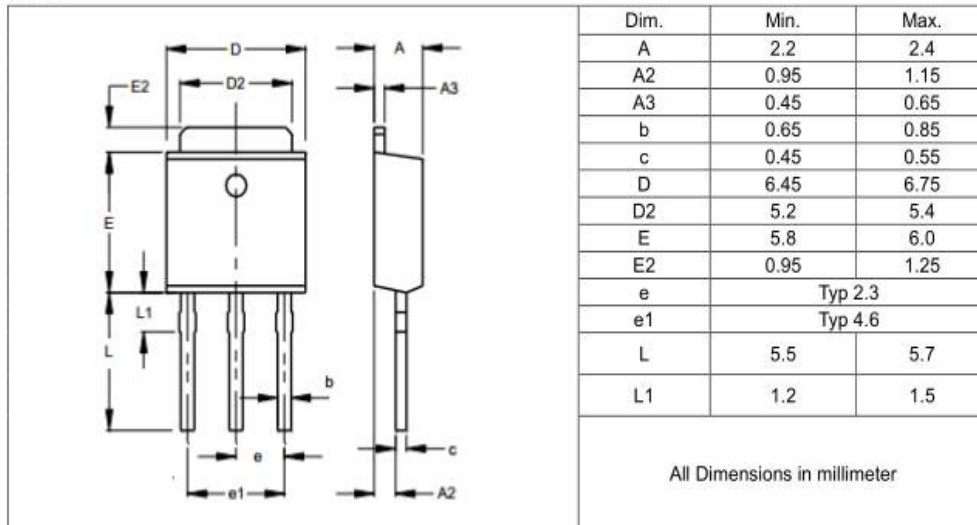
TO-251
